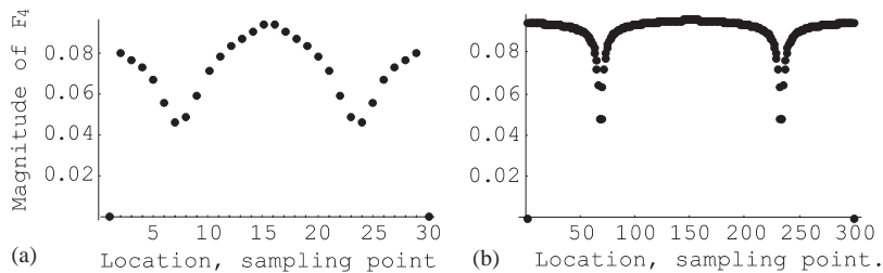
Fig. 2. Numerical estimate of F_4 for the first mode of a free–free beam: (a) n = 30, L = 1 ; (b) n = 300, L = 1 .
